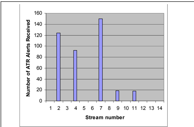
Fig 6. ATR alerts successfully detected; Stream 7 uses a CPU reservation and Diffserv Priority
