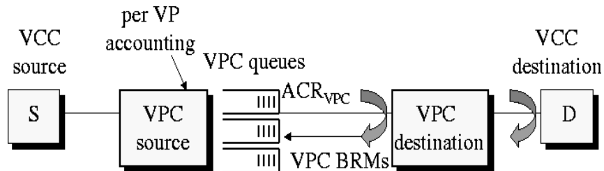
Figure 7: VPC/VCC flow control coupling without VS/VD
