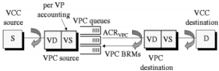
Figure 6: Virtual source/virtual destination at the VPC endpoints
