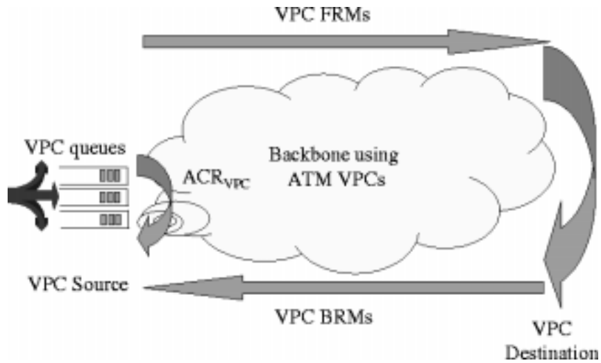
Figure 5: ABR VPCs can be used in the network backbones to minimize delay and loss.
