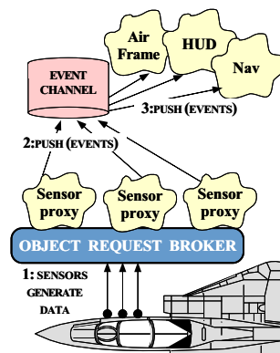
Figure 1: Example Avionics Mission Computing Application
